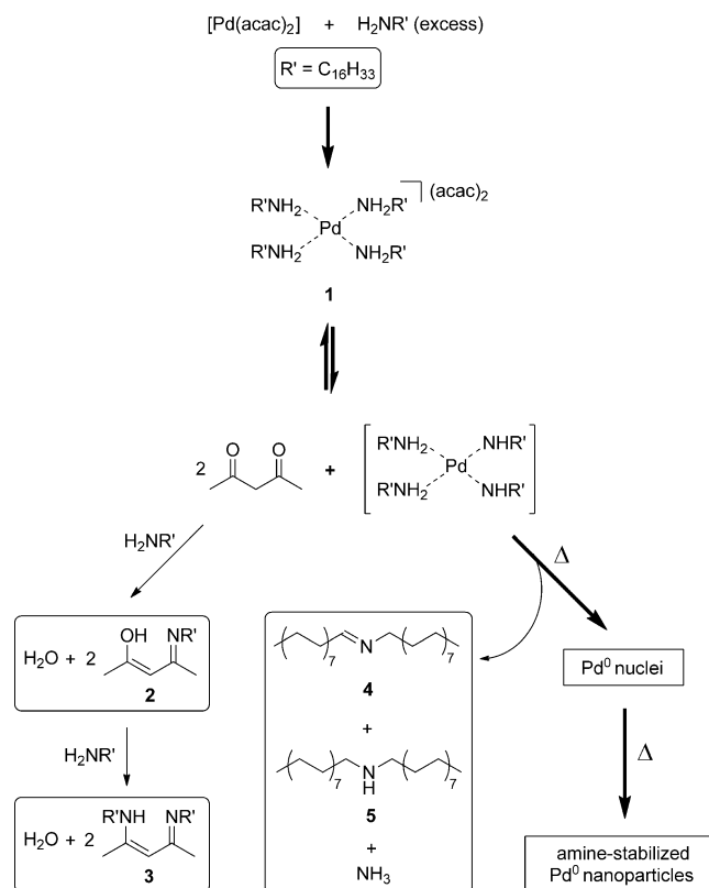
Scheme 1. Proposed mechanism for the formation of Pd 0 nanoparticles from [Pd(acac) 2 ] and a primary amine.
